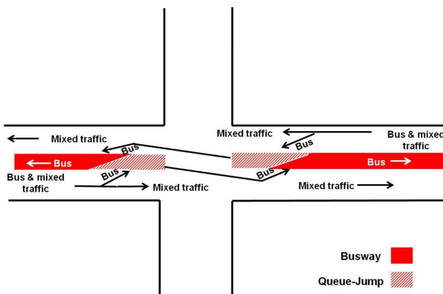
Figure XX: Virtual busways can be utilized in restricted or narrow road widths to provide dedicated right of way for BRT.
